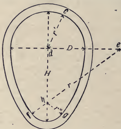
FIG. 2.—EGG-SHAPED SEWER.
